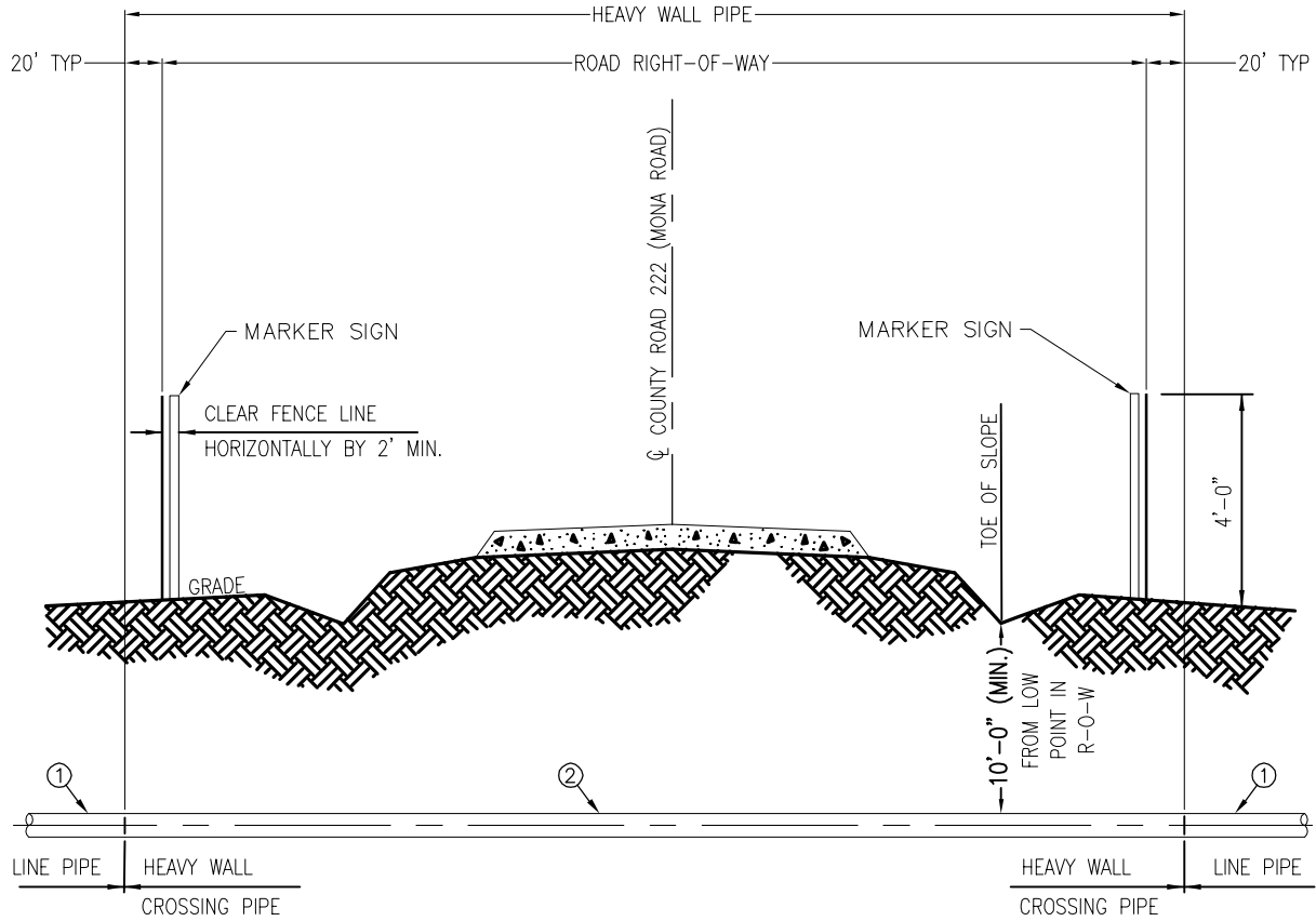
TYPICAL BORED ROAD CROSSING UNCASSED
